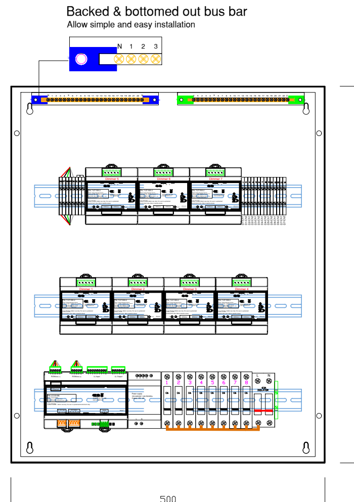
7x Trailing edge dimmer (14 channels) Size: H600 x W500 x D125
